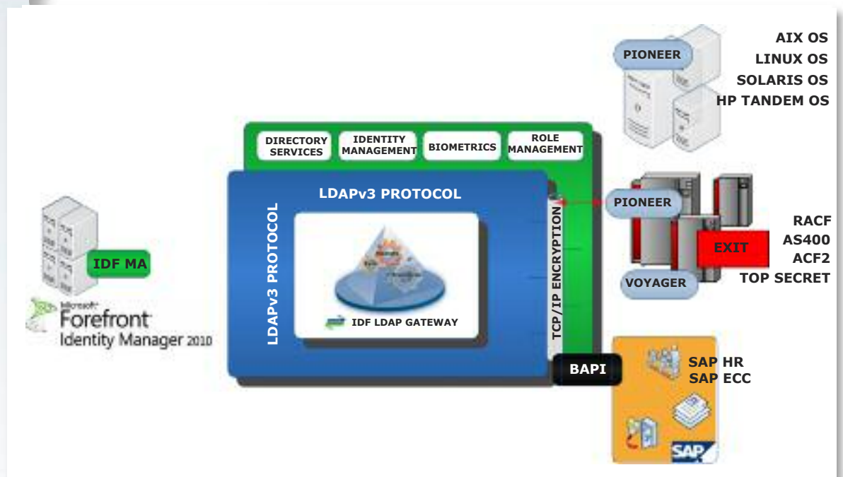
Figure 1.0 IdentityForge FIM MA Overview
